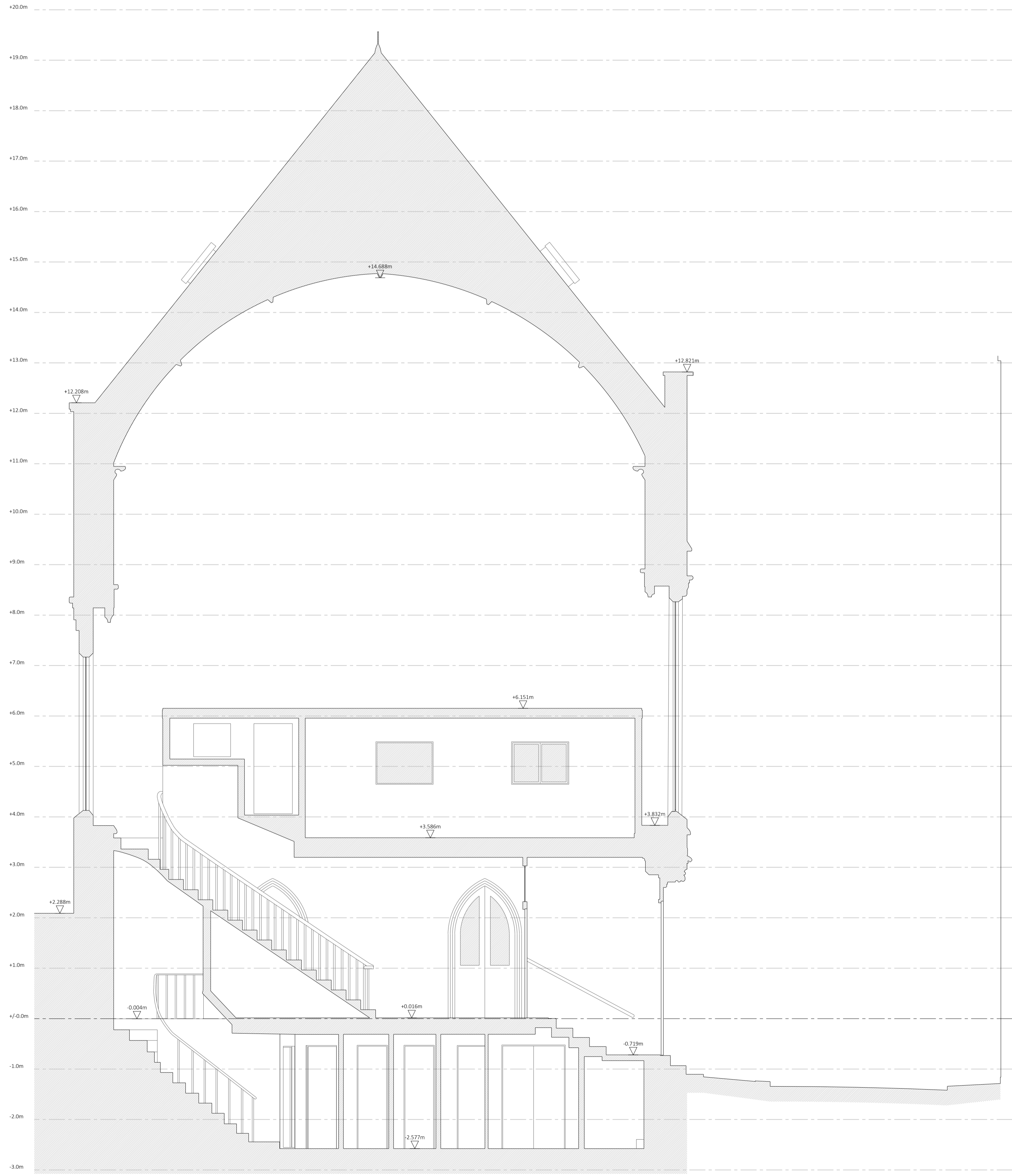
Section - S2
